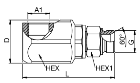
Male / Female Thread
